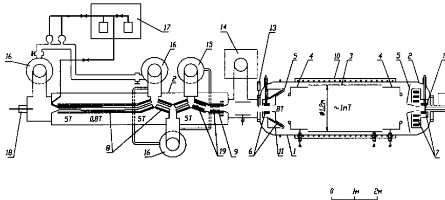
Figure 1. Schematic view of Troitsk \nu -mass set up. 1, 2 vacuum tank; 3, 4 electrostatic analyzer; 5 grounded electrode; 6, 7, 8, 9 superconducting coils; 10 warm coil; 11 N 2 jacket; 12 Si(Li) detector; 13 fast shutter; 14 Ti-pump; 15, 16 Hg diffusion pump; 17 T 2 purification system; 18 electron gun; 19 argon pump.
